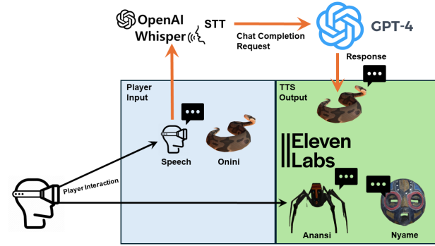
Figure 1: System architecture of the Player-NPC interaction model. Player speech is converted to text using Whisper, and GPT-4 generates dynamic NPC responses. The orange arrows represent communication between Whisper, GPT-4, and ElevenLabs, which processes player input and converts responses into speech. ElevenLabs handles both dynamic and pre-scripted text-to-speech outputs for NPCs.
